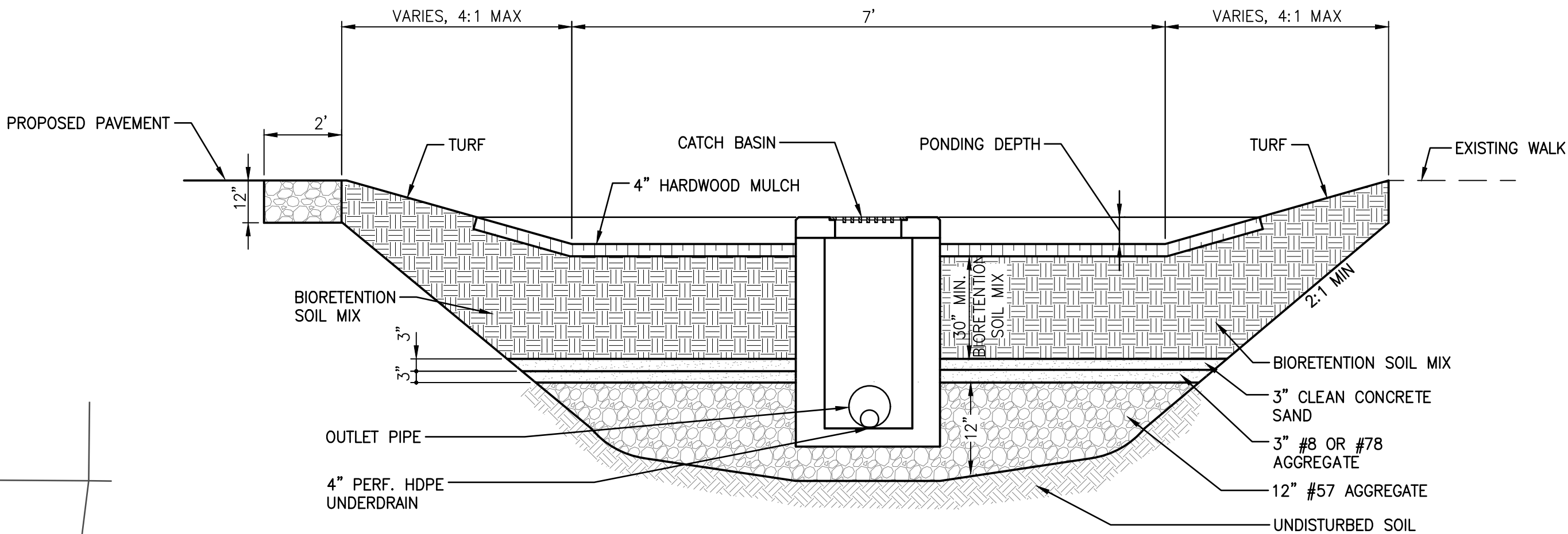
1 BIORETENTION CELL W/CATCH BASIN DETAIL 1 NOT TO SCALE
