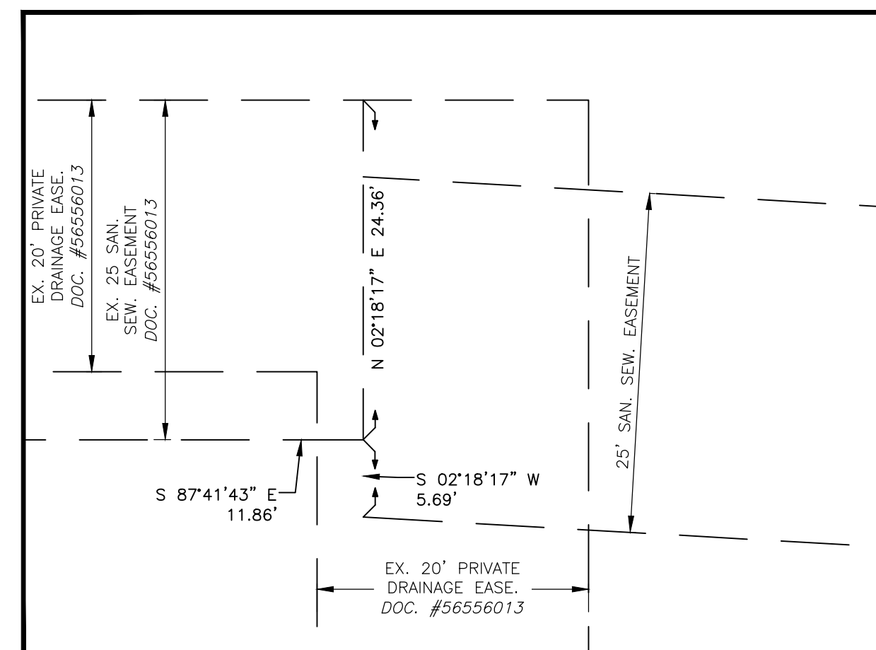
DETAIL 'A' SCALE: 1" = 10'
