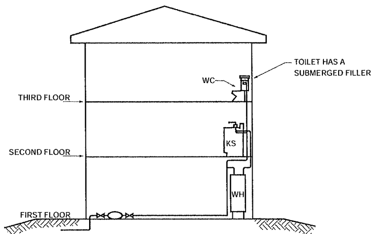
Commentary Figure 505.2(2) WATER SUPPLY PROTECTION
