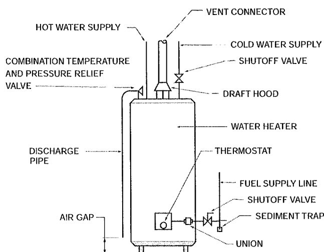
Commentary Figure 505.4 WATER HEATER INSTALLATION REQUIREMENTS
