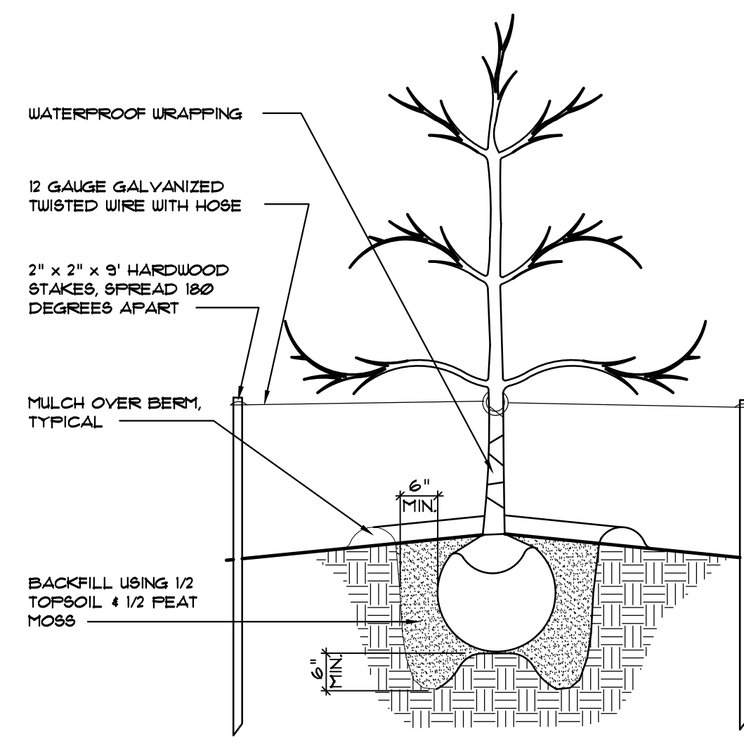
TREE PLANTING DETAIL NO SCALE
