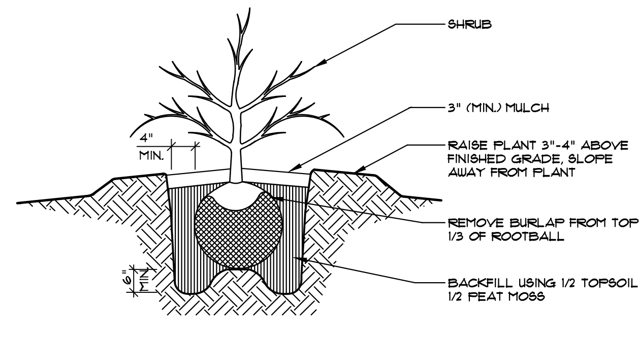
SHRUB PLANTING DETAIL NO SCALE
